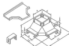
XQJ-C-04B 型上垂直四通 XQJ-C-04B Up Wards Vertical 4-Way
