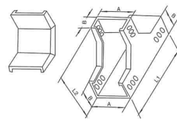
XQJ-C-03C 型下垂直三通 XQJ-C-03C Vertical Down Three-Way
