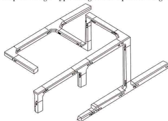
槽式桥架空间布置示意图 Sketch map of trough-type bridgeframe space arrangement
