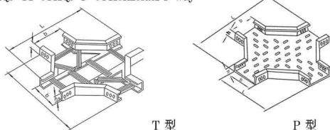
XQJ-T1-04, XQJ-P-04 型水平四通 XQJ-T1-04 XQJ-P-04 Horizontal 4-way
