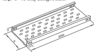
XQJ-P-01 型托盘 XQJ-P-01 Tray Bridge Frame
