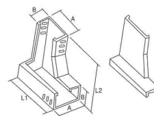
XQJ-C-05F 型垂直右下弯通 XQJ-C-05F Vertical Right-Down Wards Curved-Way
