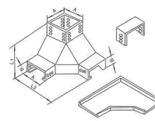
XQJ-C-03F 型上角垂直三通 XQJ-C-03F Vertical Up Three-Way
