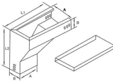
XQJ-C-05E 型垂直右上弯通 XQJ-C-05E Vertical Right-Up Wards Curved-Way
