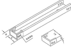
XQJ-C-01B型终端封头 XQJ-C-01B End Sealing
