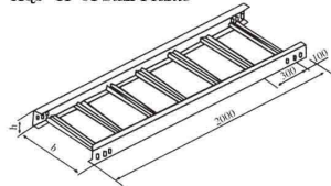
XQJ-TI-01 型梯架 XQJ-TI-01 Stair Frame
