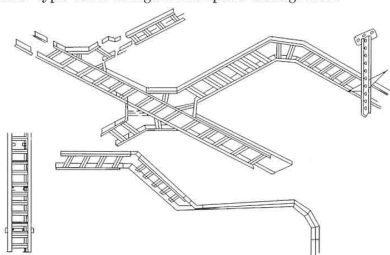
托盘式桥架空间布置示意图 Sketch map of tray-type bridgeframe space arrangement
