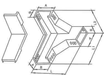
XQJ-C-03G 型下角垂直三通 XQJ-C-03G Vertical Down Three-Way
