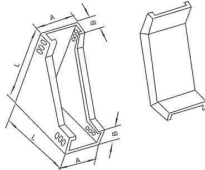
XQJ-C-05B 型垂直下弯通 XQJ-C-05B Vertical Down Wards Curved-Way
