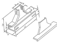
XQJ-C-03E 型下边垂直三通 XQJ-C-03E Vertical Down-Side Three-Way
