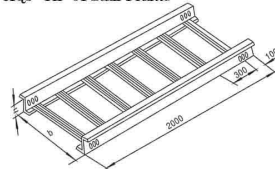
XQJ-TII-01 型梯架 XQJ-TII-01 Stair Frame
