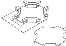
XQJ-C-04A 型水平四通 XQJ-C-04A Horizontal 4-Way
