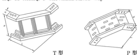
XQJ-T1-05A, XQJ-P05A 型垂直弯通 XQJ-T1-05A XQJ-P-05A Vertical Curved-Way
